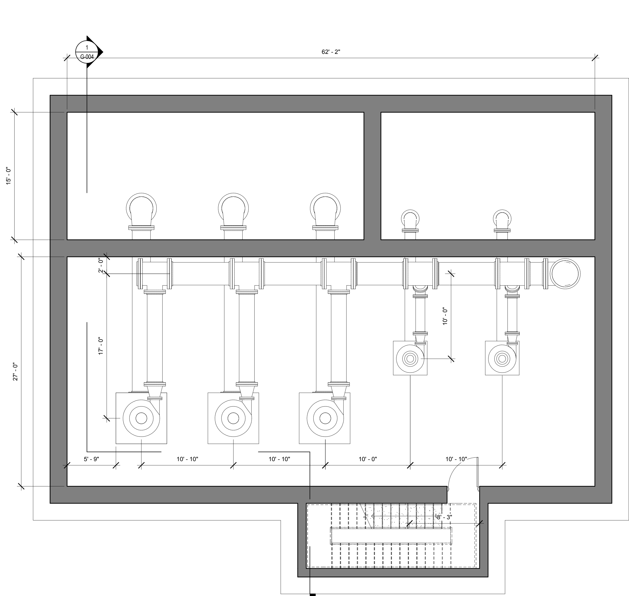
1 WET WELL LEVEL 3/16" = 1'-0"
