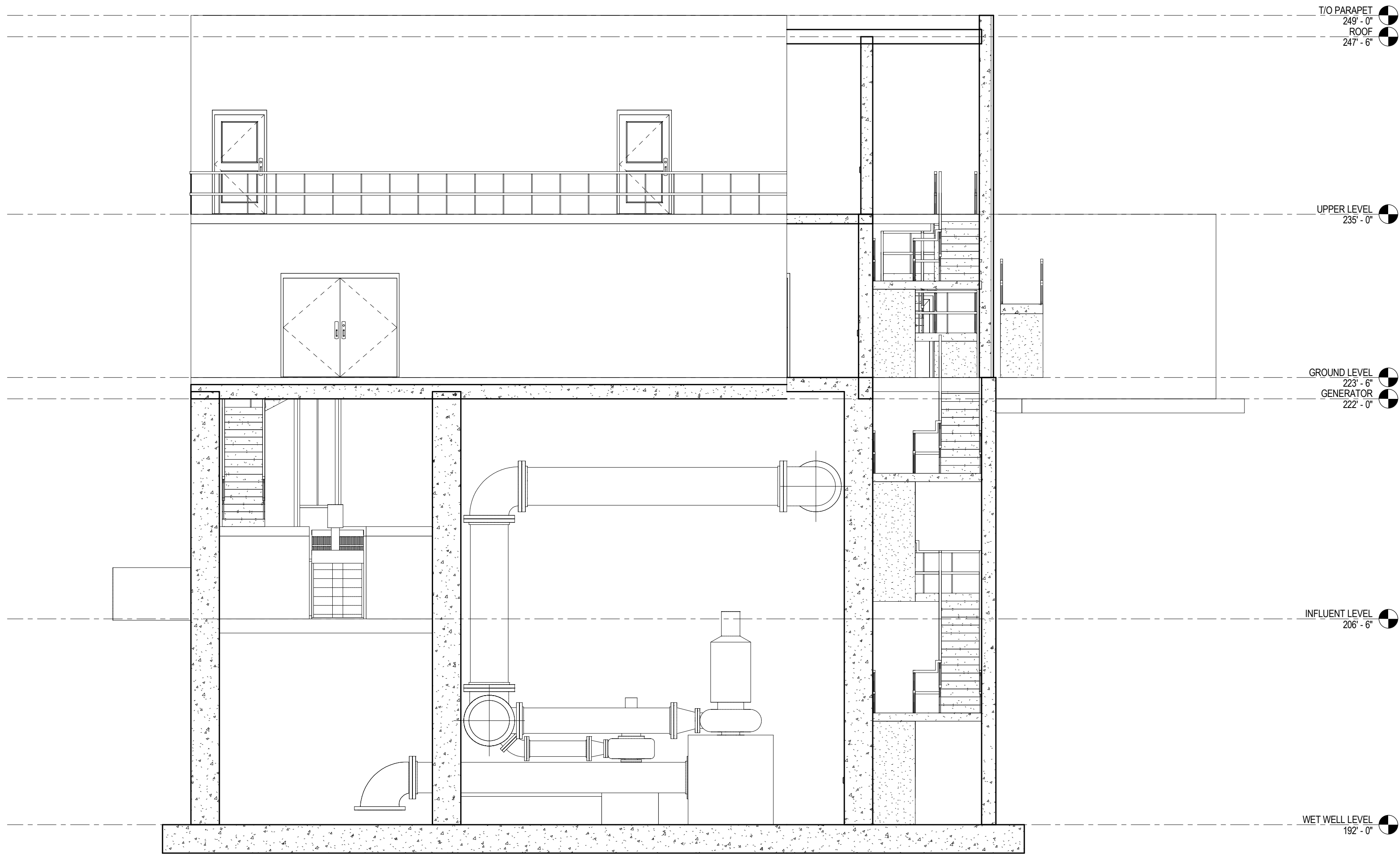
1 PARTIAL BUILDING SECTION 3/16" = 1'-0"
