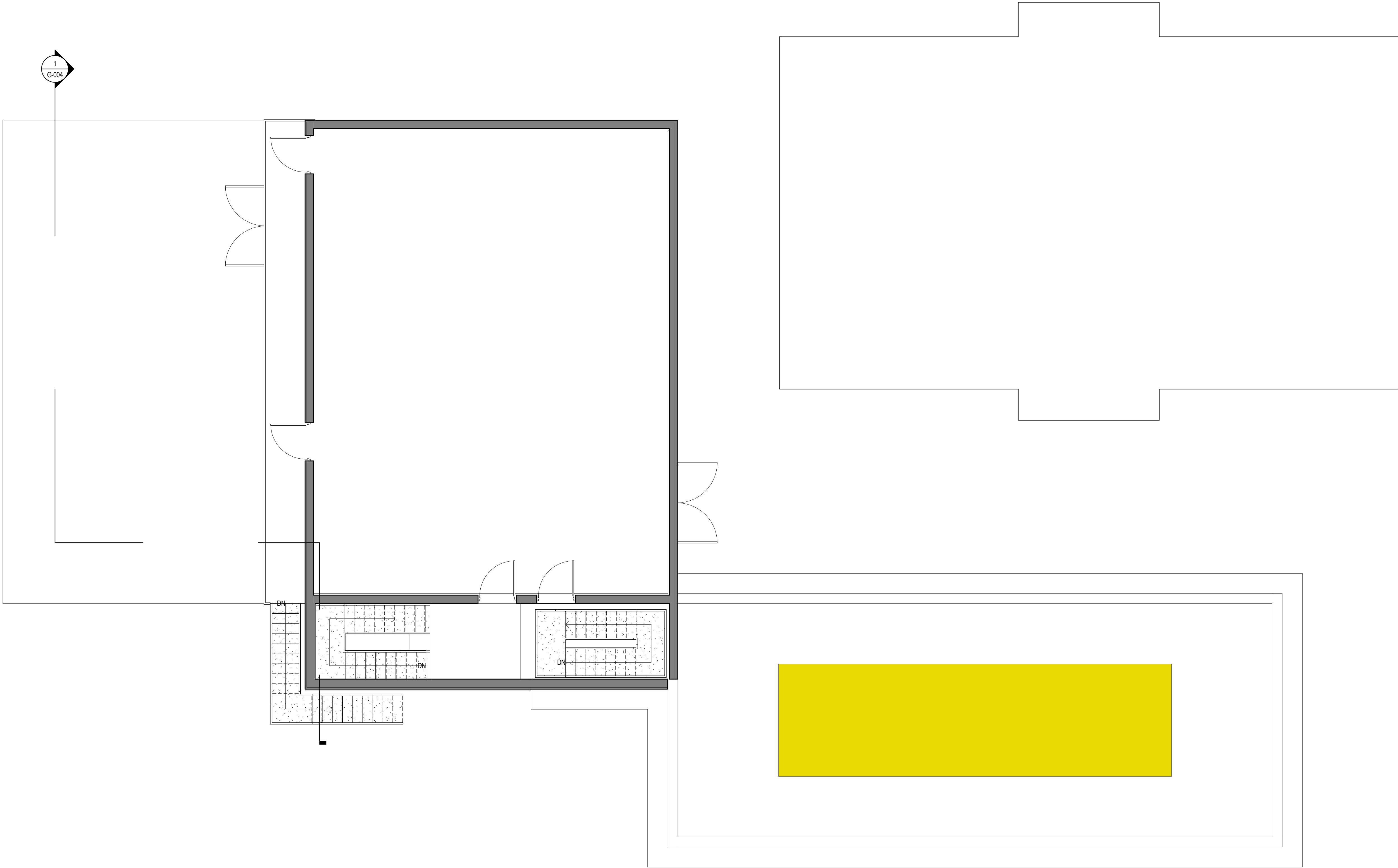
1 UPPER LEVEL PLAN 3/16" = 1'-0"
